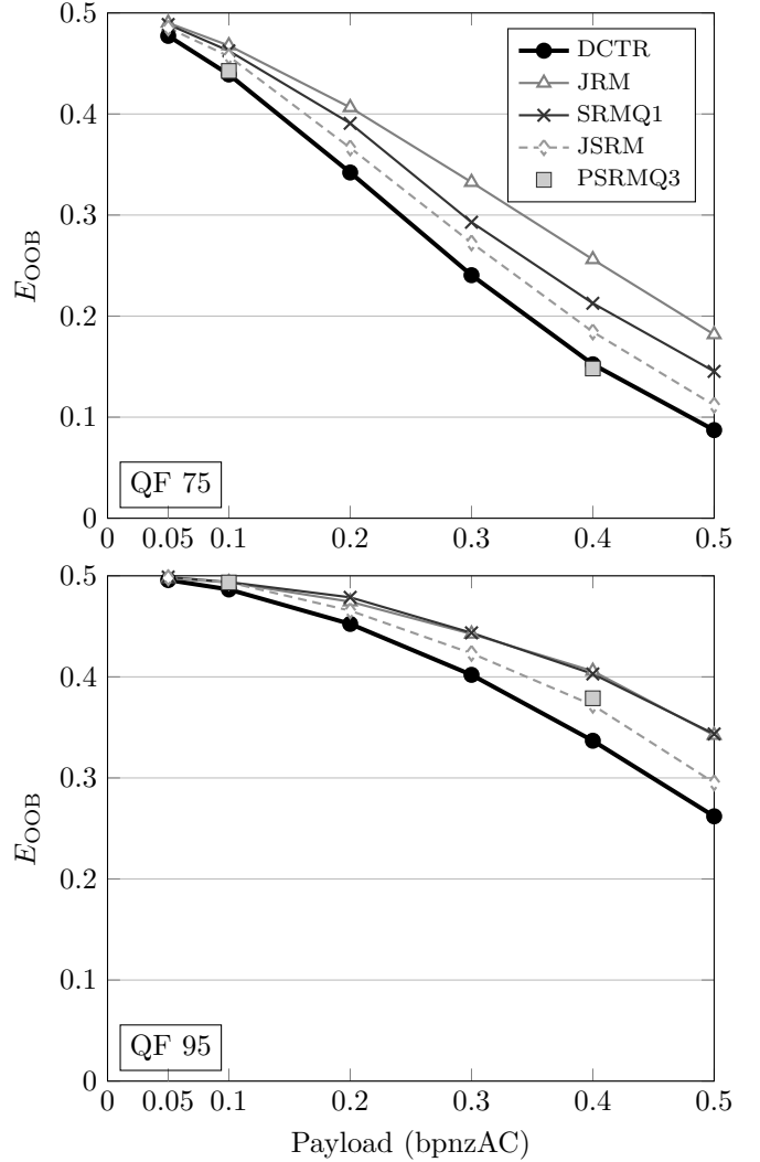
Figure 4. Detection error E_{OOB} for J-UNIWARD for quality factors 75 and 95 when steganalyzed with the proposed DCTR and other rich feature sets.
