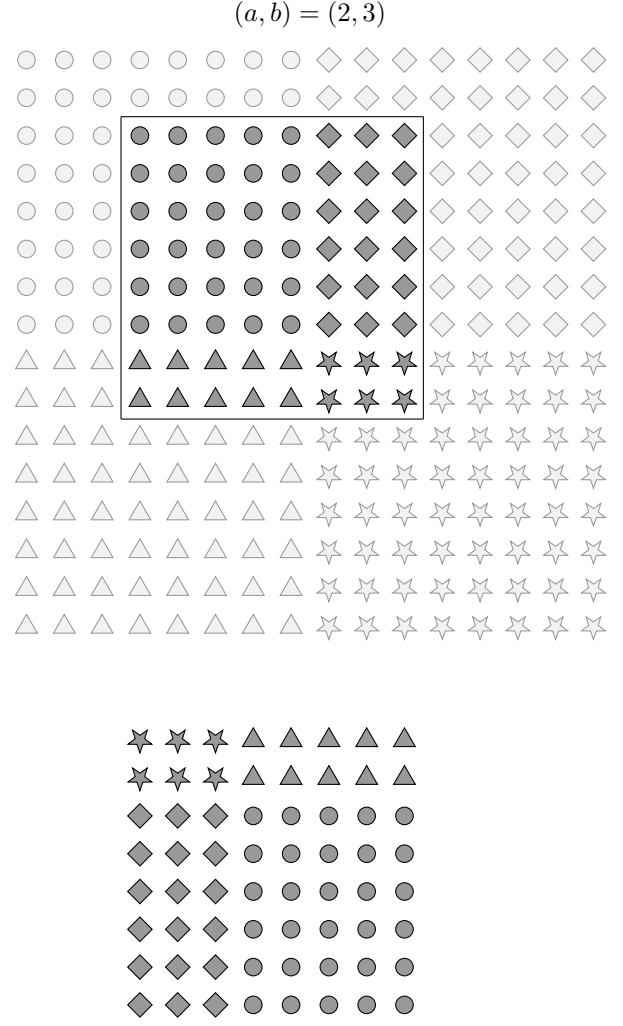
Figure 9. Diagram showing the auxiliary patterns \kappa (circle), \mu (diamond), \tau (triangle), and \sigma (star). The black square outlines the position of the DCT basis pattern \mathbf{B}^{(i,j)} .
