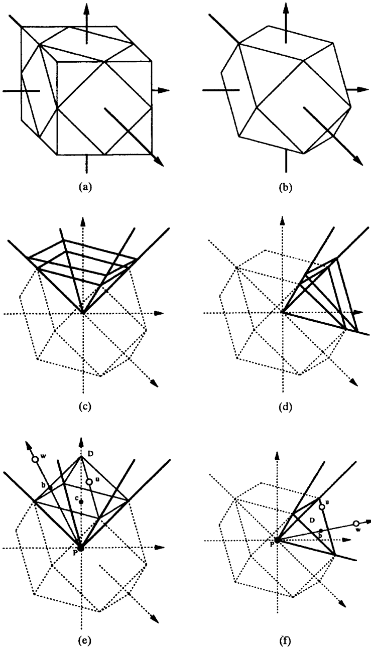
Fig. 2. A truncated cube (a), (b) induces a three-dimensional cuboctahedral partition of space into 14 regions: six square pyramids (c), and eight triangular pyramids (d). Using the triangle inequality, each region may be shown to contain at most one candidate point for connection with the origin in an MST (e), (f).
