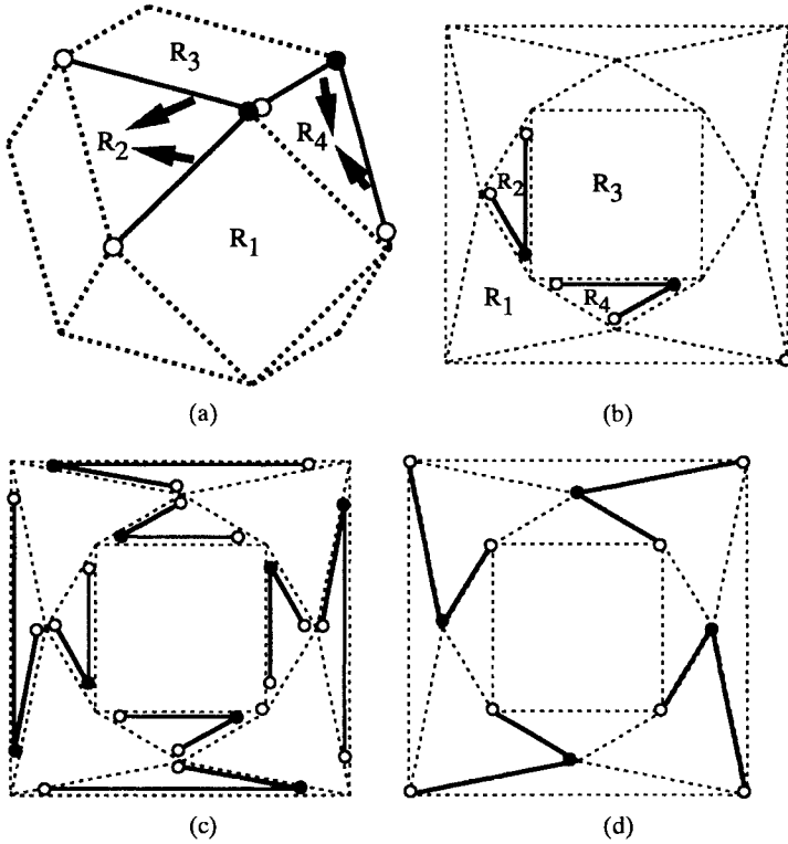
Fig. 3. Assigning the boundary points to the various regions: a hollow (solid) dot indicates an open (closed) interval. A topological mapping of the cuboctahedron (a) is shown in (b). The various boundaries are included into the triangular pyramid regions (c), while the square pyramids do not contain any boundary points. The remaining boundaries form four new regions (d), bringing the total to 18.
