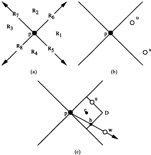
Fig. 1. A partition of \mathbb{R}^2 - \{p\} into eight regions such that for any two points u and w that lie in the same region, either \|wu\| < \|wp\| or else \|uw\| < \|up\| .
