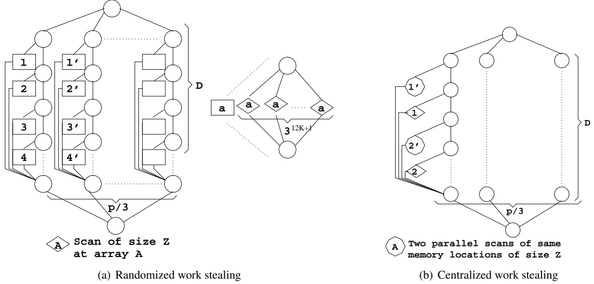
Figure 7: DAGs used in the lower bounds for randomized and centralized work stealing.
