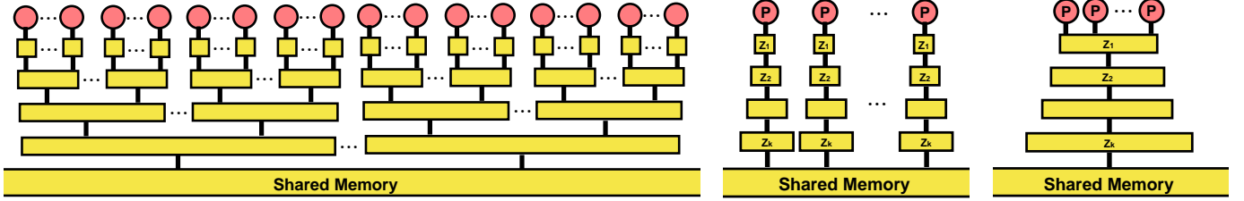
Figure 6: Left : Parallel Tree-of-Caches Hierarchy (PToC). Cache sizes and fan-out need not be regular. Center : Parallel Multi-level Distributed Hierarchy (PMDH). Right : Parallel Multi-level Shared Hierarchy (PMSH).
