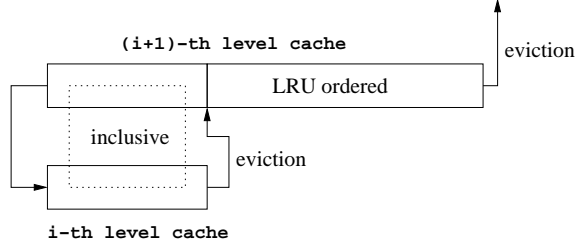
Figure 9: Multi-level LRU, depicting a parent at level i + 1 and one of its children at level i
