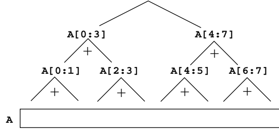
Figure 8: Prefix Sums. The first phase involves recursively summing up the elements and storing the intermediate values.
