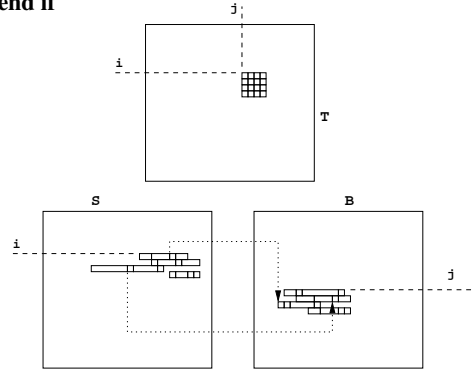
Bucket transpose diagram: The 4x4 entries shown for T dictate the mapping from the 16 depicted segments of S to the 16 depicted segments of B . Arrows highlight the mapping for two of the segments.
