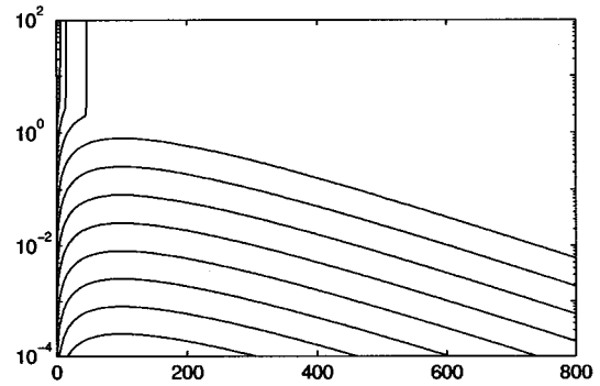
FIG. 11. Evolution curves for model (KLH) (threshold exponent \alpha=-1 ) with R=100 . This is the only figure in this paper in which no bootstrapping appears. Note that the vertical scale is shifted by two orders of magnitude; the initial amplitudes have been correspondingly shifted to \|y(0)\| = 10^{-5}, \dots, 10^0 .
