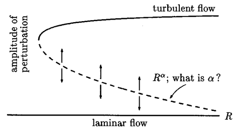
FIG. 2. Heuristic bifurcation diagram for subcritical transition to turbulence. The basin of attraction of the laminar state shrinks rapidly as R \rightarrow \infty . Small deviations from the laminar flow are enough to move the flow across the boundary into the basin of attraction of the turbulent state.
