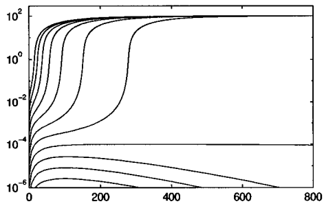
(a) Model (TTRD') (threshold exponent \alpha = -3 )
