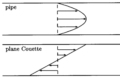
FIG. 1. Laminar velocity profiles for pipe and plane Couette flows. These solutions of the Navier–Stokes equations are stable to infinitesimal perturbations in principle for all Reynolds numbers R , but unstable in practice for large R .
