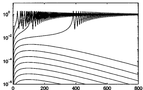
(b) Model (TTRD'') (threshold exponent \alpha = -2 )
