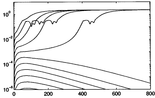
FIG. 10. Evolution curves for model (GG) (threshold exponent \alpha=-3 ) with R=100 . (For nonzero values of the advection parameter \gamma , the exponent changes to \alpha=-2 .)
