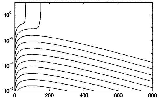
FIG. 12. Evolution curves for model (KLH') (threshold exponent \alpha=-2 ) with \sigma=1 , R=100 .
