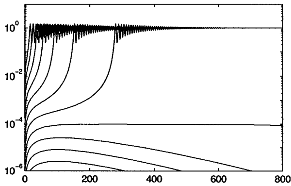
FIG. 4. Evolution curves for the model (TTRD) (threshold exponent \alpha = -3 ) with R = 100 . The curves show the vector norm \|y(t)\| for initial conditions of amplitudes \|y(0)\| = 10^{-7}, 10^{-6.5}, 10^{-6}, \dots, 10^{-2} .
