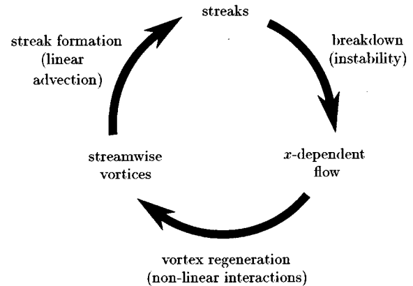
FIG. 3. Schematic illustration of the ideas underlying (a) the Marburg and Cornell models (figure taken from Ref. 7) and (b) the CTR/MIT model (figure taken from Ref. 8). Schema (a) is abstract, depending only on certain general mathematical properties, whereas schema (b) is physical, attempting to delineate the actual structures that interact in shear flows at high Reynolds number. Apart from this difference, however, these ideas correspond more closely than it may at first appear. The upper-left arrow in the CTR/MIT schema represents the dominant mechanism of what the Marburg/Cornell schema calls “linear, non-modal growth,” and the other two arrows amount to a proposal of a dominant mechanism of “nonlinear mixing.” It might appear that the division of this latter part of the loop into two arrows—breakdown followed by regeneration—represents a fundamental difference between (a) and (b), but this is not so. When “nonlinear mixing” is modeled by arbitrary quadratic interactions among variables, these two phases usually still emerge, for reasons explained in Sec. IX.
