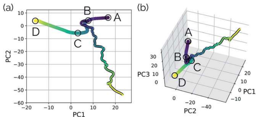
Fig. 8 MD trajectory for fluoride dissociation projected into the reduced dimensional space defined by the IRC for the S_{\text{N}}2 system with respect to (a) the top two principal components and (b) the top three principal components. The IRC, as in previous plots, is shown by the purple to yellow color-mapped line and the trajectory is shown with the same color-mapping, but a black outline. The equivalent plots for PCA on the aligned Cartesian coordinates can be found in the ESI.†
