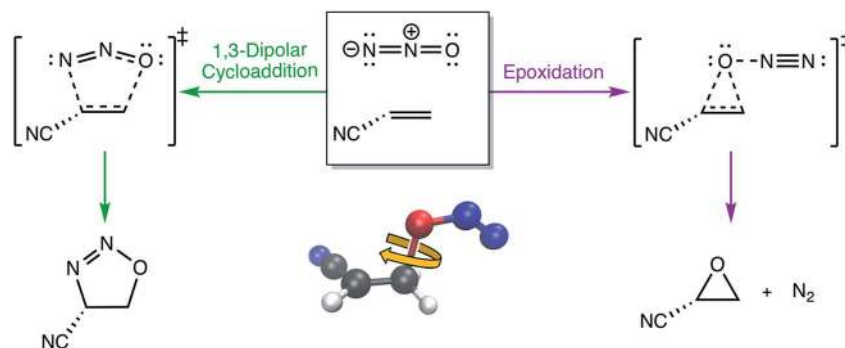
Fig. 9 The two possible pathways of \text{N}_2\text{O} reacting with acrylonitrile. The ball-and-stick inset illustrates the dihedral angle rotation of the \text{N}_2\text{O} –acrylonitrile complex that appears to be the primary geometric coordinate that differentiates the two transition state structures along the competing pathways.
