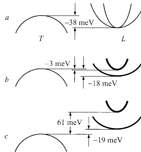
Figure 2. Schematic energy band diagram showing the energies of the subband edges for the heavy and light electrons and for the holes for: (a) bulk Bi, (b) 100 nm diameter Bi nanowires along the bisectrix direction, and (c) 50 nm diameter Bi nanowires along the bisectrix direction.
