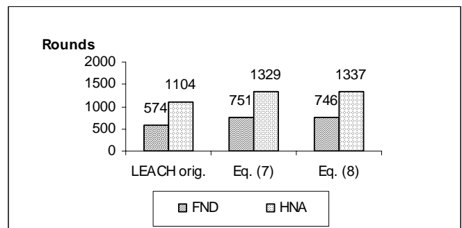
Fig. 2. Simulation results of the sample network with the base station located at (100,300). LEACH's original cluster-head selection algorithm is compared with the modifications denoted by Eq. (7) and (8).
