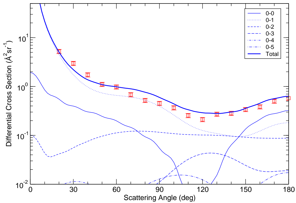
Figure 1. Elastic (rotationally summed) DCS of water at 4 eV. The squares are the experimental points from Cho et al (2003). The present calculation is given by the thick solid line. Other lines denote partial state-to-state DCS.
