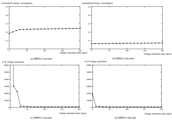
Figure 6: The normalized energy consumption and the number of voltage transitions of the AVS-converted MPEG-4 encoder and decoder program.
