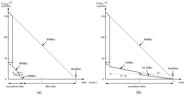
Figure 3: The changes of C_{RWEC}(t) over different speed scaling algorithms: (a) no intra-task scheduling and (b) RWEC-based intra-task scheduling.
