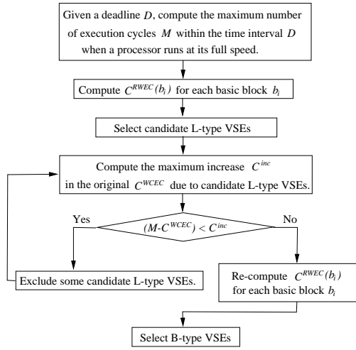
Figure 4: Overall VSE selection algorithm.
