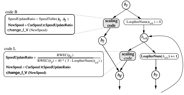
Figure 5: Code generation for VSEs.
