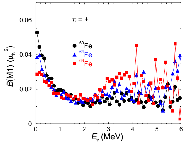
FIG. 1: (Color online) Average B(M1) values in 100 keV bins of transition energy calculated for positive-parity states in ^{60}\text{Fe} (black circles), ^{64}\text{Fe} (blue triangles up), and ^{68}\text{Fe} (red squares).
