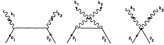
FIG. 2. The lowest-order perturbation-theory contributions to Compton scattering on a spinless target.
