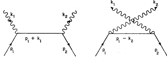
FIG. 3. The lowest-order perturbation-theory contributions to Compton scattering on a spin- \frac{1}{2} target.
