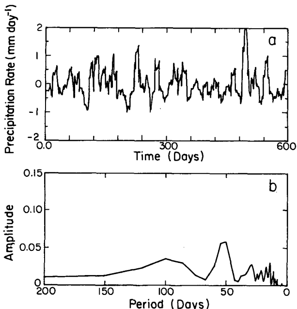
FIG. 8. (a) Simulated precipitation rate (in mm day -1 ) from a 600-day segment of a run with a “complete” version of model 2. (b) Spectral analysis of the precipitation record shown in (a).
