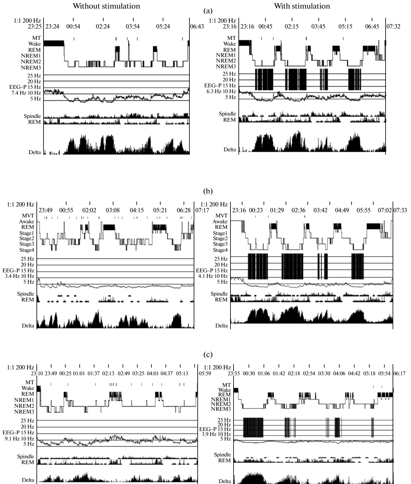
Fig. 2. Hypnograms and EEG spectral characteristics obtained in three different subjects (a) M.I.; (b) Sh.D.; (c) M.V.) during the nights with and without stimulation in sleep stages 3–4. The vertical lines on the hypnograms (to the right) mark the electrical impulses. Y axis top-down, time scale, sleep stages, averaged power for all EEG channels and all frequency bands; sleep spindle hypnograms, eye movement histograms, power spectrum of EEG delta band. X axis (above), time.
