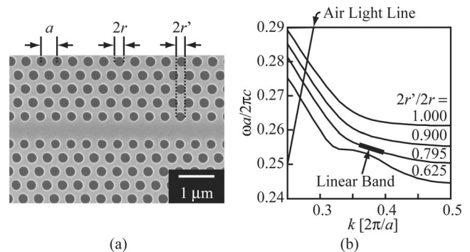
Fig. 1. Device structure and photonic band. (a) Top view of LVL PCW fabricated on SOI substrate. (b) Photonic band of the main propagation mode of PCW for 2r/a=0.667 . 2r'/2r is taken as a parameter.
