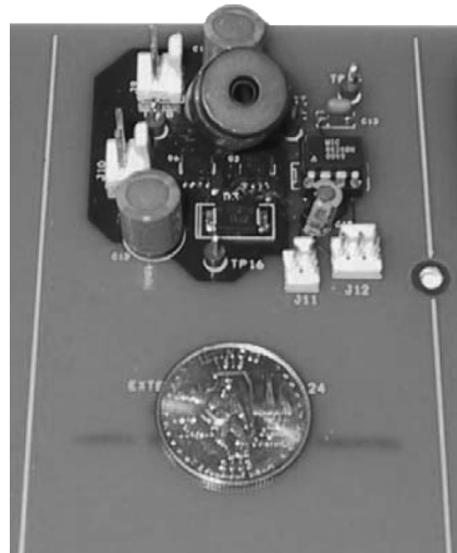
Fig. 2. Photograph of 3-W (nominal) low-input-voltage converter.
