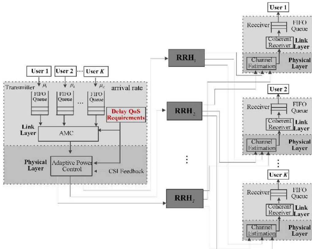
Fig. 2. The statistical QoS provisioning over the 5G C-RAN.
