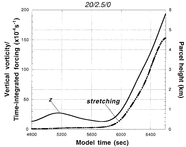
FIG. 9. Time series of parcel height ( z ; km) and time-integrated contribution to vertical vorticity from the relative vorticity-stretching term [ s^{-1} ; see Eq. (4.1)], along the forward trajectory denoted as “F” in Fig. 6.
