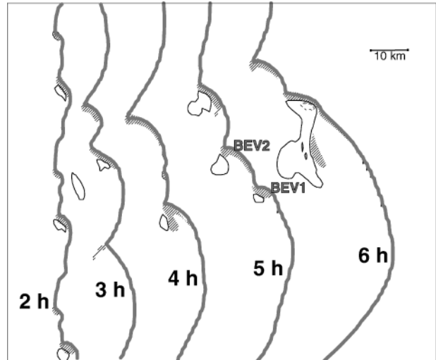
FIG. 17. Ground-relative horizontal wind magnitude (bold dark lines, 35 \text{ m s}^{-1} contour; thin dashed line, 40 \text{ m s}^{-1} contour) at z = 0.127 km, over the interval 2 \leq t \leq 6 h. Stippled regions enclose vertical vorticity values greater than or equal to 0.008 \text{ s}^{-1} . The bold gray line indicates the -1\text{-K} perturbation temperature isotherm. Only a 100 \text{ km} \times 100 \text{ km} portion of the full domain is shown.
