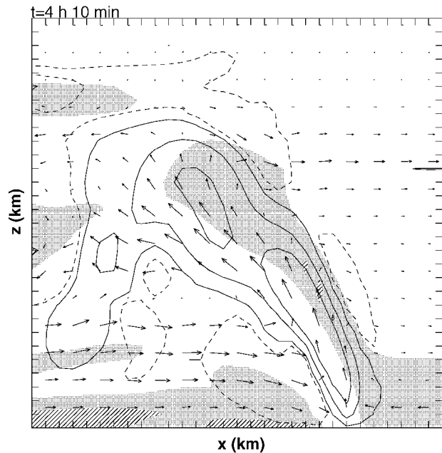
FIG. 15. West-east vertical cross section through the apex of the primary bowing segment at t = 4 \text{ h } 10 \text{ min} . Contours are of vertical velocity ( -0.5, 1, 5, 10 \text{ m s}^{-1} ). The stippled regions enclose y-component horizontal vorticity between 50 and 150 \times 10^{-4} \text{ s}^{-1} and the hatched regions enclose y-component horizontal vorticity greater than 150 \times 10^{-4} \text{ s}^{-1} . Vectors are of velocity in the x-z plane. Every second vector is plotted, and the vector length is scaled so that a distance of two grid lengths in the horizontal or vertical represents a vector magnitude of 15 \text{ m s}^{-1} . The horizontal (vertical) subdomain is 30 \text{ km} ( 15 \text{ km} ).
