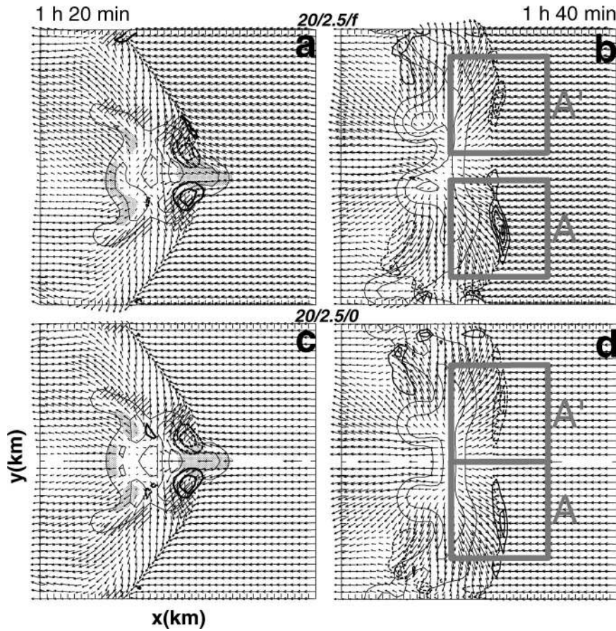
FIG. 5. Horizontal velocity vectors, the 1, 3, and 5 g kg -1 rainwater contours (thin lines), and vertical vorticity contours (bold lines; contour interval of 0.004 s -1 ) at z = 0.4 km. (a), (b) The 20/2.5/f simulation at t = 1 h 20 min and 1 h 40 min, respectively. (c), (d) The 20/2.5/0 simulation at t = 1 h 20 min and 1 h 40 min, respectively. The vector length is scaled so that a horizontal distance of 1 km represents a speed of 10 m s -1 . In (a) and (d), the stippled regions enclose vertical velocities less than or equal to -5 m s -1 at z = 3 km, and the hatched regions enclose vertical velocities greater than or equal to 10 m s -1 at z = 3 km. In (b) and (d), the gray boxes represent control areas A and A' (see text). Only a 40 km × 40 km portion of the full domain is shown.
