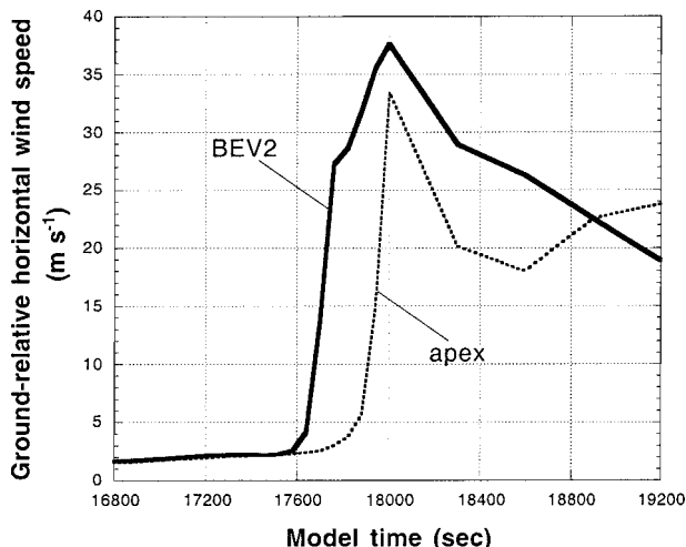
FIG. 18. Time series of ground-relative wind ( \text{m s}^{-1} ) at ground-fixed points affected by BEV2 and the bow-echo apex at t = 5 h (see Fig. 16).
