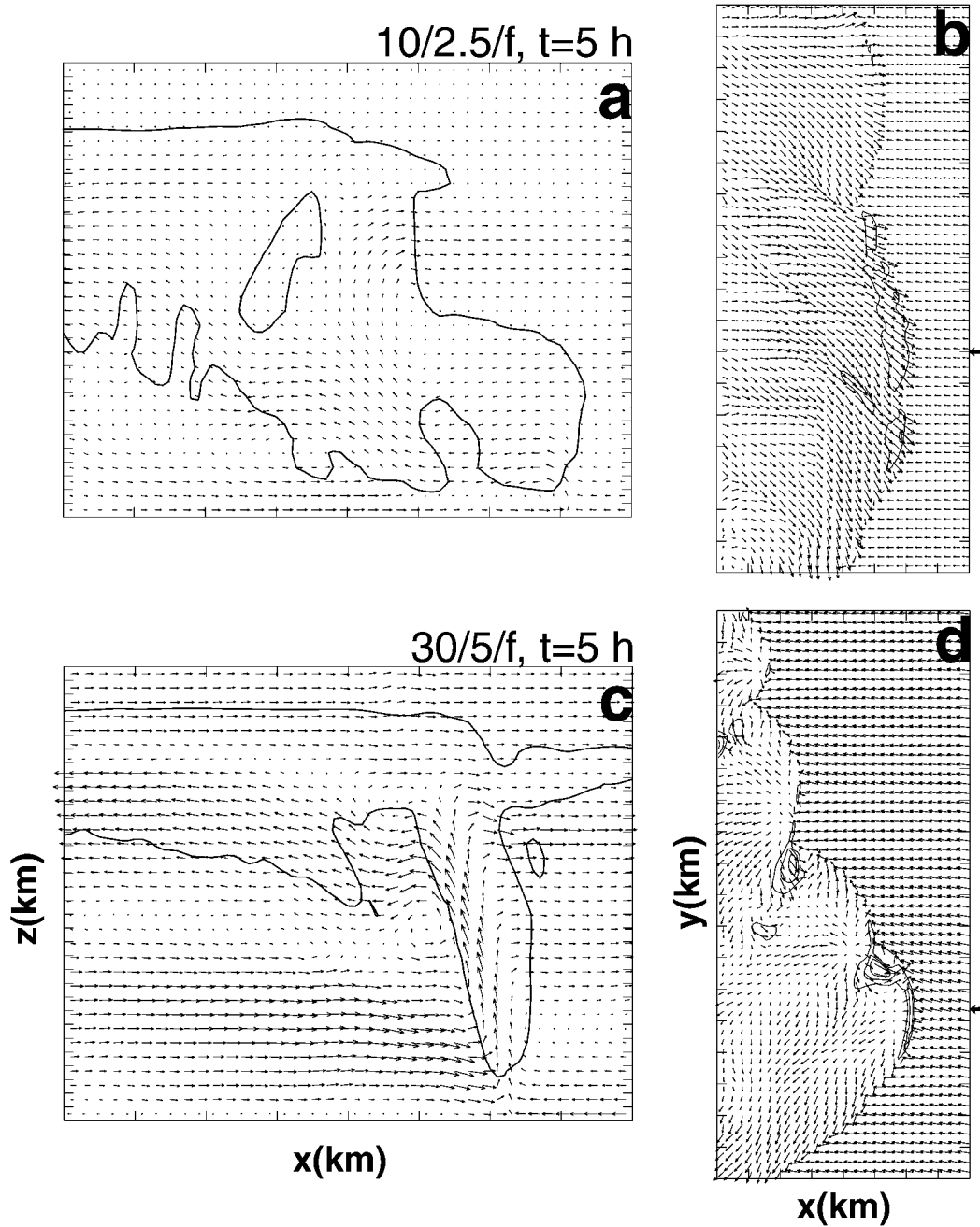
FIG. 20. Vertical and horizontal structure, at t = 5 h, of the convective systems simulated with (a), (b) 10/2.5/f and (c), (d) 30/5/f . In (a) and (c), vertical cross sections of north–south-averaged [centered about y = 70 km and y = 54 km, respectively, as indicated in (b) and (d)] wind vectors and cloud water mixing ratio ( 0.1 \text{ g kg}^{-1} contour) are presented. In (b) and (d), horizontal cross sections, at z = 0.127 km, of horizontal velocity vectors and the 30, 35, and 40 \text{ m s}^{-1} contours of ground-relative horizontal wind magnitude are presented. Only an 80 \text{ km} \times 16 \text{ km} ( 80 \text{ km} \times 180 \text{ km} ) portion of the full domain is shown in (a) and (c) [(b) and (d)].
