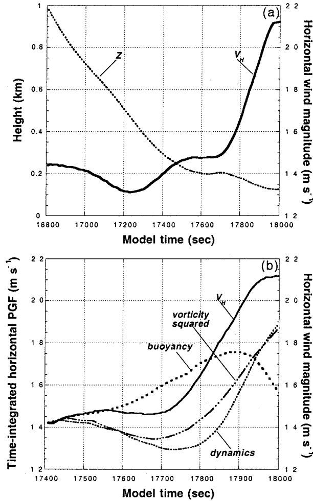
FIG. 19. (a) Time series of height [ z (km); dotted line] and horizontal wind magnitude [ V_H ( \text{m s}^{-1} ); solid line] along the trajectory indicated in Fig. 16. (b) Time series of V_H and of the time-integrated horizontal pressure-gradient force owing to “buoyancy” ( -c_p \bar{\theta} \partial \pi_B / \partial s ), “dynamics” ( -c_p \bar{\theta} \partial \pi_{DN} / \partial s ), and “vorticity squared” ( -c_p \bar{\theta} \partial \pi_{\zeta}^2 / \partial s ) along part of the trajectory represented in (a). “Horizontal” here is the horizontal direction locally parallel to the trajectory (see text). Wind magnitude at t = 4 h 50 min is added to the time-integrated pressure-gradient force terms to allow for comparison with V_H . Note that the time domain of (b) is half that of (a).
