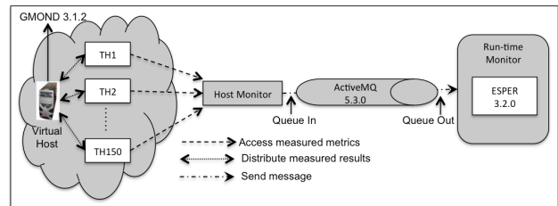
Figure 4. Evaluation Testbed
