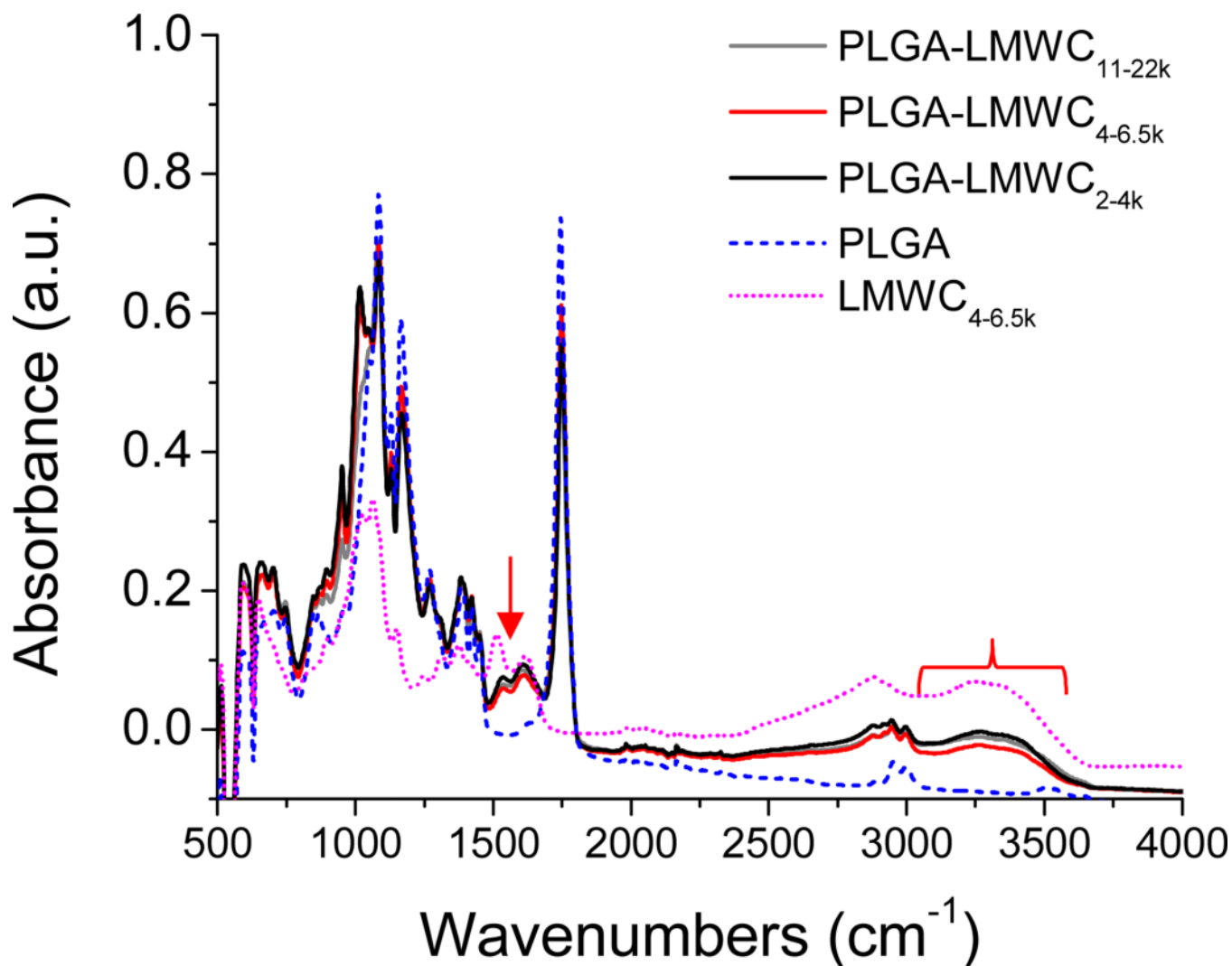
Fig. 2. FTIR spectroscopy of PLGA-LMWCs, PLGA and LMWC 4-6.5k . The presence of amide and amine bands (arrow, 1500–1690 \text{cm}^{-1} ) and a broad N-H signal (brace, 3000–3700 \text{cm}^{-1} ) confirms the conjugation of LMWC to PLGA.
