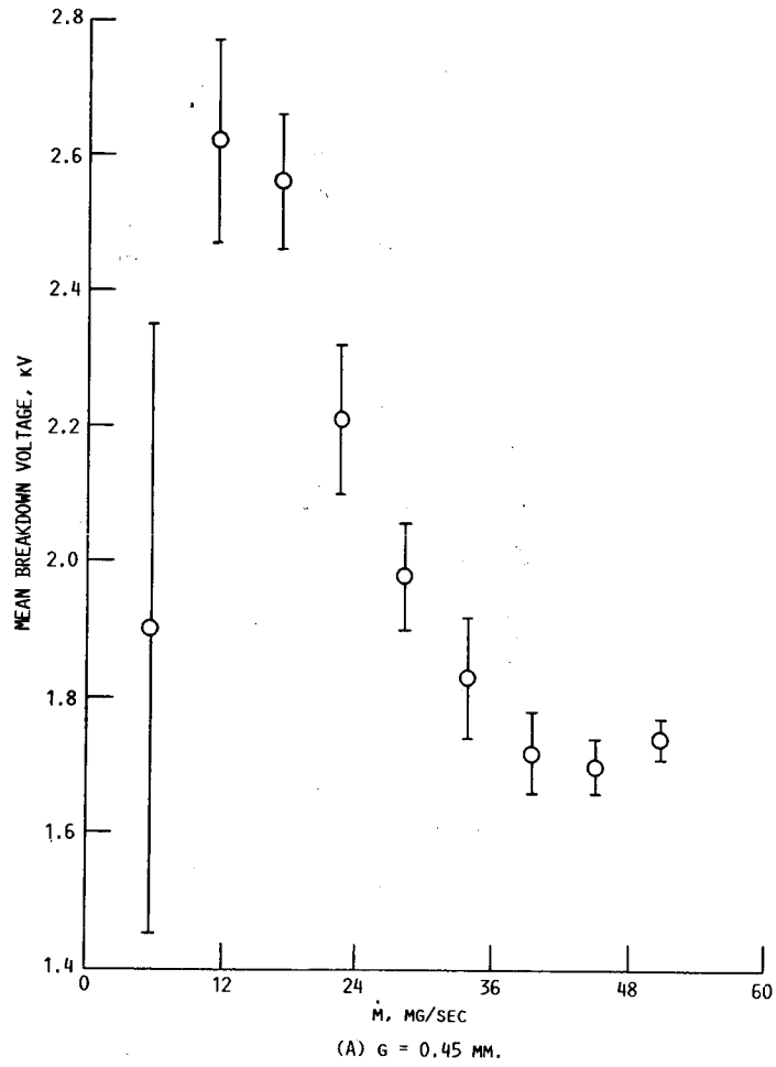
FIGURE 9. - MEAN BREAKDOWN VOLTAGE (BDV) VERSUS MASS FLOW, M OF 1:2 MOLE RATIO N_2:H_2 GAS MIXTURE FOR PULSE P1 FOR VARIOUS GAP SETTINGS, g. BARS REPRESENT \pm 1\sigma IN BDV DISTRIBUTION FOR 100 SPARKS.
