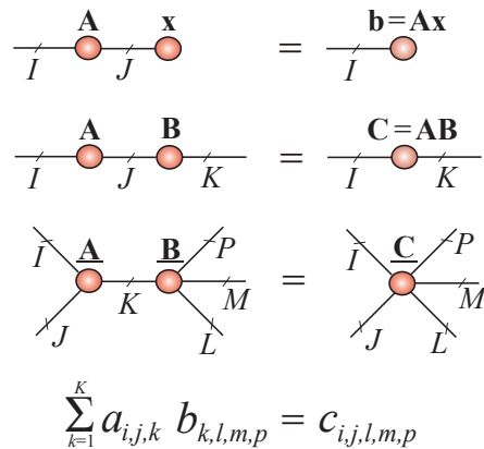
Figure 1.5: Graphical representation of tensor manipulations. (a) Basic building blocks for tensor network diagrams. (b) Tensor network diagrams for matrix-vector multiplication (top), matrix by matrix multiplication (middle) and contraction of two tensors (bottom). The order of reading of indices is anti-clockwise, from the left position.
