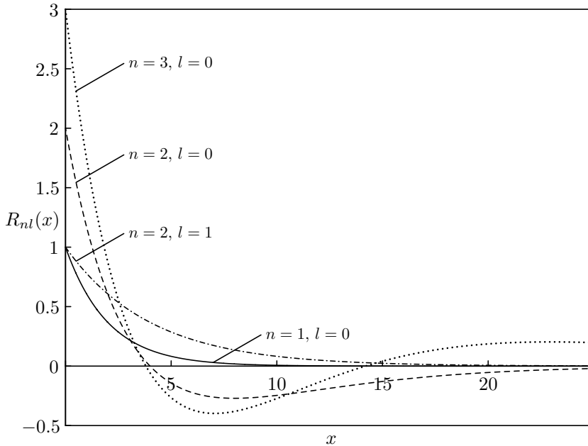
Figure 5. Radial parts of the first four HLO functions.
