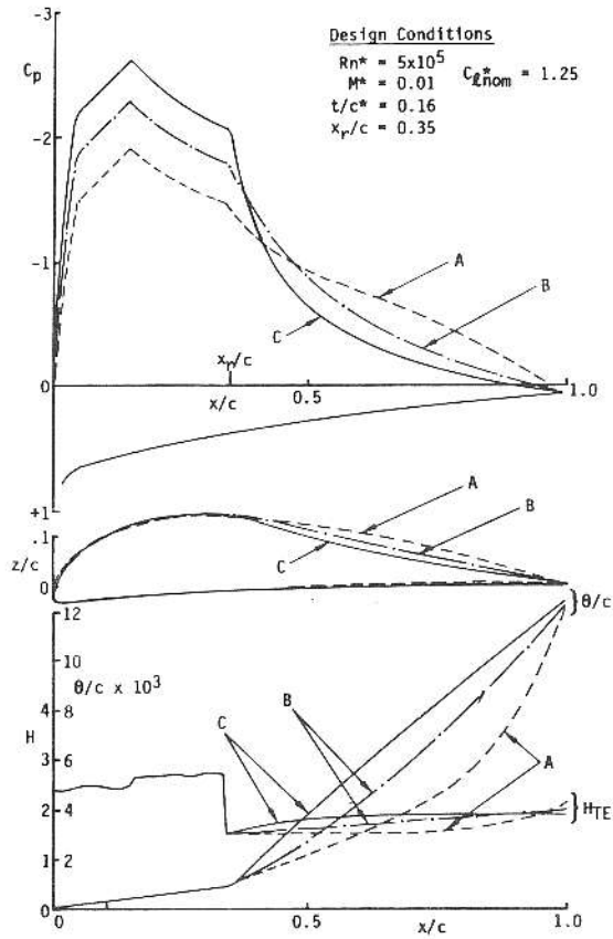
FIGURE 17 THREE AIRFOILS DESIGNED FOR THE SAME LIFT COEFFICIENT AT Re = 5 \times 10^5
