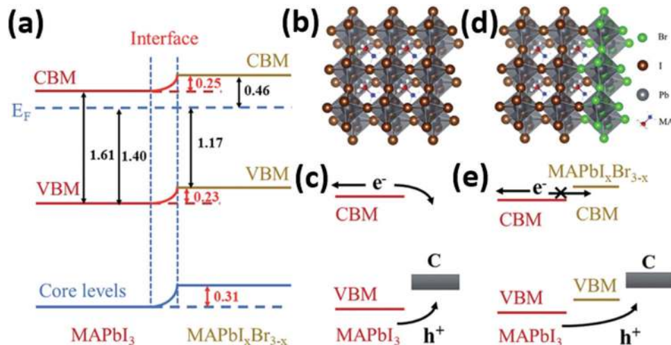
Fig. 27 (a) Energy level diagram of the stacked MAPbI 3 /MAPbI x Br 3-x perovskite interface. (b) Crystal structure and (c) charge transfer diagram at the MAPbI 3 /carbon electrode interface. (d) Crystal structure and (e) charge transfer diagram of the stacked MAPbI 3 . Adapted and reprinted with permission from ref. 217.
