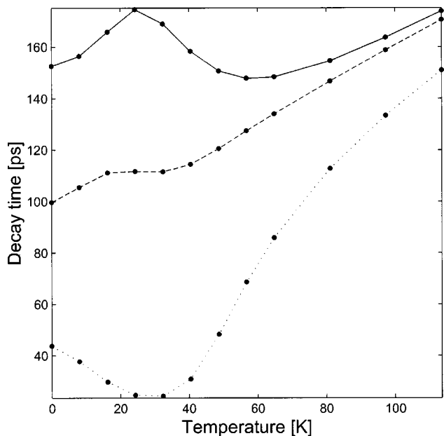
FIG. 8. Temperature dependence of the fluorescence decay time \tau_e(E_d) calculated for aggregates of N=250 molecules, with J=600 \text{ cm}^{-1} , \gamma_0=2 \times 10^{-3}J , \sigma=0.3J , and W_0=100J . The data were obtained by numerical solution of Eq. (6) under the condition of off-resonance blue-tail excitation. The dots mark the numerical data, while the lines connecting the dots are guides to the eye. The three curves correspond to different detection energies E_d related to the steady-state fluorescence spectrum in Fig. 4(b): detection at the position of the red half maximum of this spectrum (solid line), at the peak of this spectrum (dashed line), and at the blue half maximum (dotted line). The average was performed over 10 000 realizations of the disorder.
