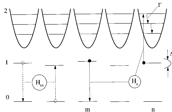
FIG. 1. Schematic representation of all interactions contributing to the exciton–exciton annihilation process. The interaction H_{ex} , indicated by the dashed lines, forms excitonic states in the subspace of the molecular states ‘‘0’’ and ‘‘1.’’ Excitons annihilate through a high-lying electronic-vibrational molecular term ‘‘2’’ ( \omega_{10} \approx \omega_{21} ). The first step of the annihilation process results from the intermolecular interaction H_a , which induces simultaneous transitions of the molecule m to the ground state and molecule n to the high-lying term. The second step results from fast vibrational relaxation within high-lying electronic-vibrational sublevels towards the ground vibrational state characterized by a rate \Gamma \gg H_a .
