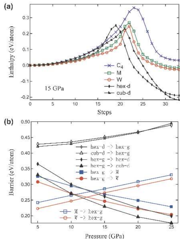
FIG. 3: (color online). (a) Enthalpy versus pathway at 15 GPa for the transformations shown in Fig. 2. (b) Enthalpy barriers versus pressure. The solid and open symbols represent the reaction and counter-reaction barriers, respectively.
