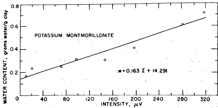
c. Potassium-montmorillonite.
