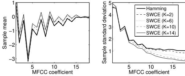
Fig. 3. Multitapers help in reducing variance of the higher-order MFCCs, but without modifying the mean value much.
