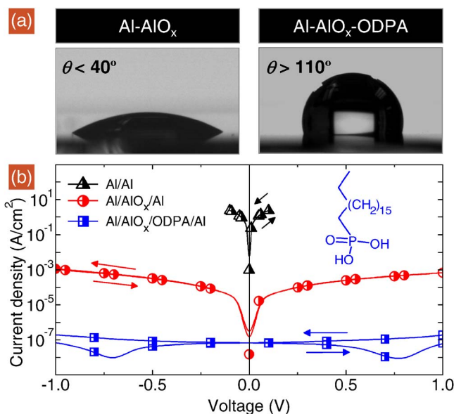
FIG. 1. (Color online) (a) Water droplets on Al-AIO x (left) and on Al-AIO x -ODPA (right). (b) Current density vs bias voltage for diodes fabricated with untreated Al electrodes (triangles), oxidized bottom electrode (circles) and ODPA functionalised Al-AIO x bottom electrode (squares). Inset: molecular structure of ODPA.
