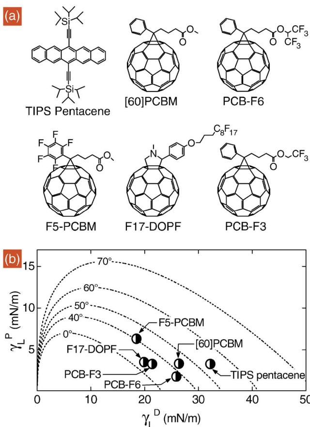
FIG. 2. (Color online) (a) Chemical structure of the molecules studied. (b) Wetting envelopes for the AIO x -ODPA surface with coordinates of liquid surface energy components of semiconductor solutions plotted (symbols).
