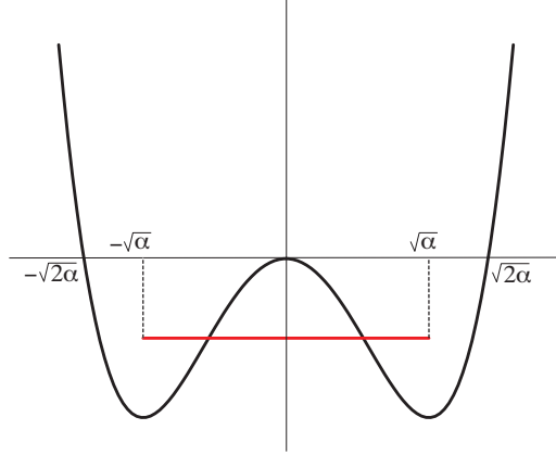
FIG. 2. Functions f (black) and g (red) of Example 7.2 .
