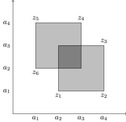
FIG. 1. Corresponding to Example 7.1 : in light grey, the separately convex hull of \{z_i\}_{i=1}^6 ; in dark grey, the square [a_2, a_3] \times [a_2, a_3] .
