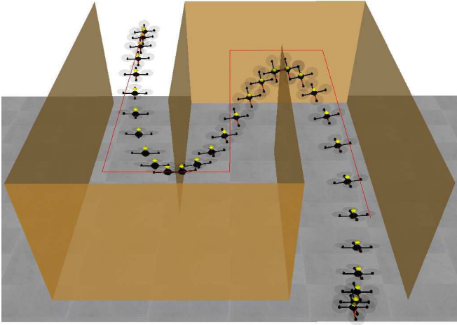
Fig. 7. The S-Maze scenario for our quadrotor simulation experiments. The thin red line is the guiding path. The quadrotor is shown at 6Hz. Videos are available at http://gamma.cs.unc.edu/CA/LQGObs/ .
