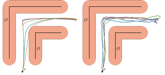
Fig. 5. Controlling the robot (see Section V-B) using LQG-Obstacles in the same environment as Fig. 3. (a) Traces of maximum likelihood executions for \bar{p} = \{0.01, 0.02, 0.03, 0.05, 1\} . (b) Traces of five actual executions with synthetic motion and observation noise for \bar{p} = 0.01 .
