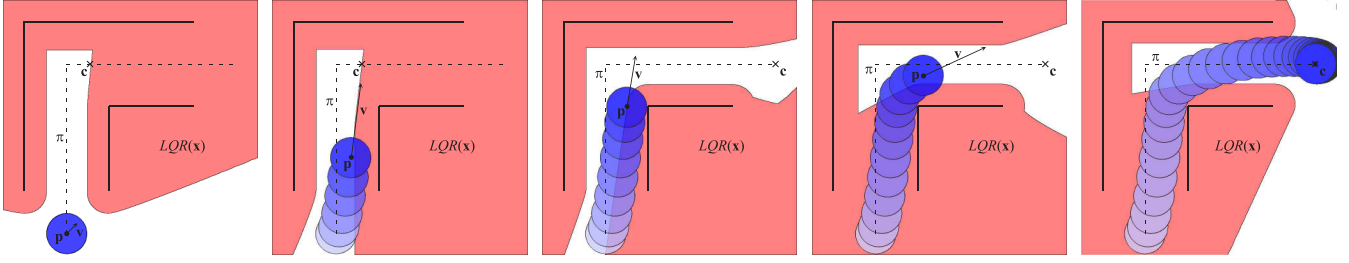
Fig. 3. Navigating a circular robot whose acceleration can be controlled (see Section V-B) through a narrow corridor using LQR-Obstacles. The workspace obstacles are shown using thick lines. The guiding path \pi is shown by a dashed line. In each frame, the LQR-Obstacle \mathcal{LQR}(\mathbf{x}) for the particular state \mathbf{x} = (\mathbf{p}, \mathbf{v}) is shown. The valid configuration \mathbf{c} farthest along the guiding path is chosen as target configuration.
