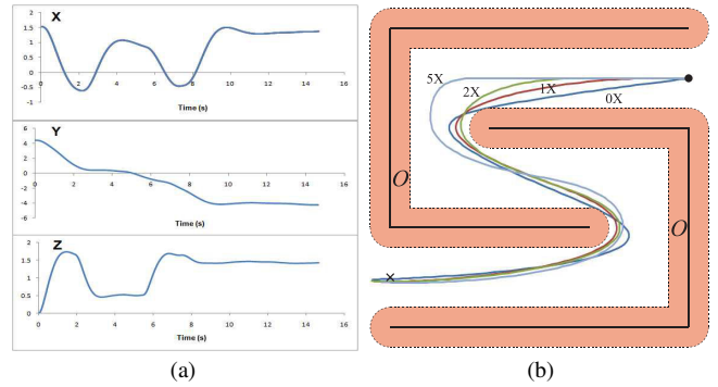
Fig. 8. (a) The x , y , and z position over time of the quadrotor in the 3-Window scenario (see Fig. 1). (b) The xy -projections of the maximum likelihood traces of the quadrotor in the S-Maze scenario (see Fig. 7) for 0, 1, 2, and 5\times the realistic amount of uncertainty.
