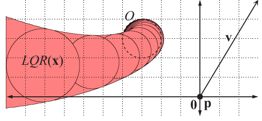
Fig. 2. The LQR-Obstacle \mathcal{LQR}(\mathbf{x}) shown as a union of transformed configuration-space obstacles for a planar robot of which the acceleration can be controlled (see Section V-B) with current state \mathbf{x} = (\mathbf{p}, \mathbf{v}) . The configuration-space obstacle \mathcal{O} is a disc shown by the dashed circle. The LQR-Obstacle consists of all target configurations \mathbf{c} that result in a collision when an LQR controller is used to control the robot to that configuration.
