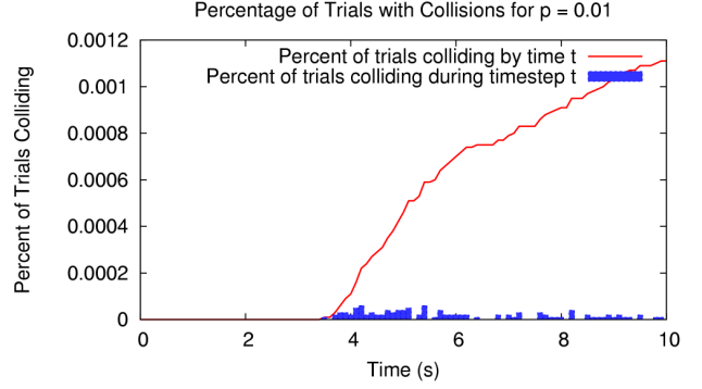
Fig. 6. Probability of collision over time for the LQG-Obstacle with \bar{p} = 0.01 .
