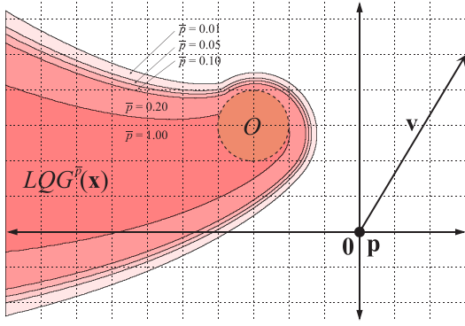
Fig. 4. The LQG-Obstacle \mathcal{LQG}^{\bar{p}}(\hat{\mathbf{x}}) in the same configuration as in Fig. 2 accounting for motion and sensing uncertainty of the robot (see Section V-B). The conservative approximation of Eq. (25) is shown for various values of the probability bound \bar{p} . For \bar{p} = 1 , it is equivalent to the LQR-Obstacle.
