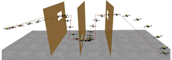
Fig. 1. The 3-Window scenario for our quadrotor simulation experiments. The red line is the guiding path. Our approach smoothly controls the quadrotor (shown at 4Hz) through the windows without colliding with the walls. Videos are available at http://gamma.cs.unc.edu/CA/LQGObs/ .
