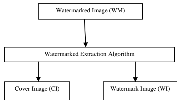
Figure 3.2 Watermark Extraction
