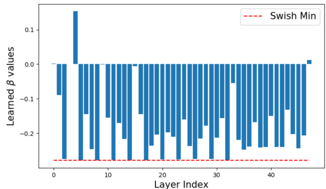
Figure 2. Layerwise \beta values after coverage for EfficientNet-B0
