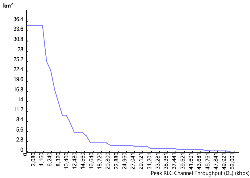
FDD – 2100 Covered area / Throughput (DL)
