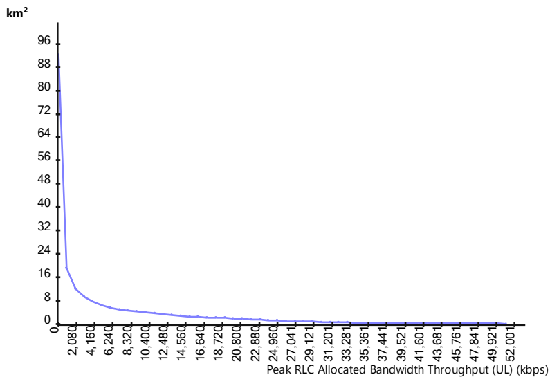
FDD – 2100 Covered area / Throughput (UL)
