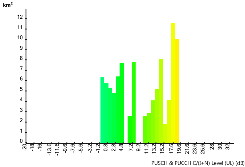
TDD – 2100 Covered area / Carrier-to-noise ratio (UL)
