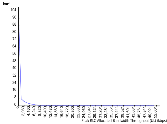
TDD – 2100 Covered area / Throughput (UL)
