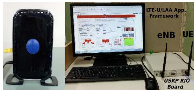
Fig. 3. Equipment used in the testbed: (i) Netgear N600 wireless dual band router WNDR3400v3 used as Wi-Fi AP. (ii) USRP RIO board with LTE-U eNB and LTE-U user operated using LTE-U/LAA Application framework.
