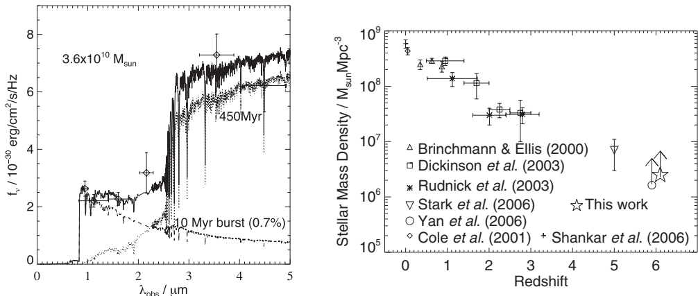
Figure 3. Left: the spectral energy distribution from Spitzer /IRAC and HST data for a z \sim 6 star-forming galaxy (Eyles et al. 2005). If we fit two stellar populations (ongoing star formation and an older burst), we find that there are stars as old as 450 Myr at z \approx 6 (within 900 Myr of the Big Bang). This pushes the formation epoch back to z \sim 10 , around the time to reionization. Right: The assembly of stellar mass at high redshift, derived from Spitzer measurements of Lyman break galaxies (Eyles et al. 2007). Our high redshift points are lower limits because the Lyman break selection only picks out actively star-forming galaxies (and not post-burst systems).
