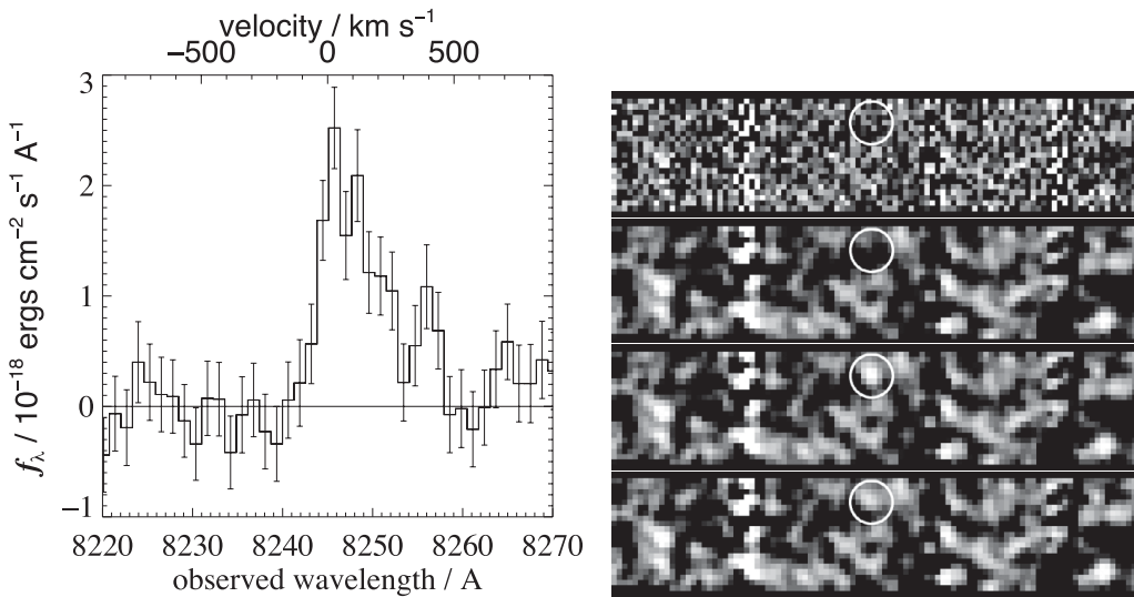
Figure 5. Left: A growing subset of the z \approx 6 Lyman break population have been spectroscopically confirmed through Lyman- \alpha emission (figure from Bunker et al. 2003). At higher redshifts, z > 7 , the spectroscopy has been less successful, perhaps because the resonant Lyman- \alpha line is absorbed by optically-thick neutral hydrogen in the Inter-Galactic Medium during the Gunn-Peterson era.
