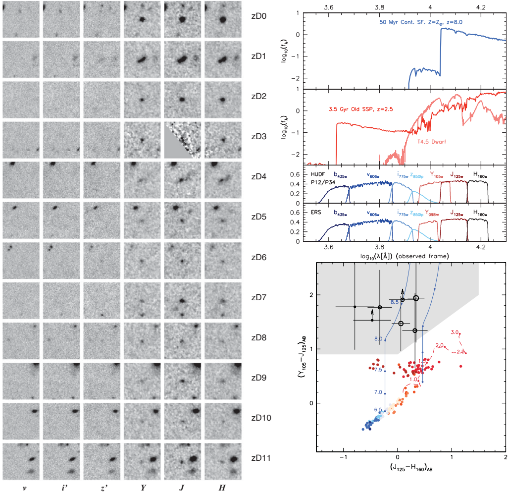
Figure 1. Left: The z' -band dropouts at z \sim 7 identified in the WFC 3 and ACS imaging of the Hubble Ultra Deep Field (Bunker et al. 2010). The top candidate, zD0, is actually an intermediate-redshift supernova (rather than a high redshift Lyman break galaxy) which occurred during the more recent WFC 3 imaging from 2009 but was absent in the 2003 ACS images.
