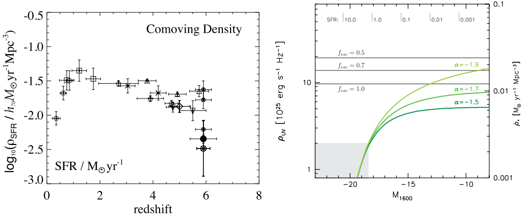
Figure 4. Left: the evolution of the star formation rate density (the “Madau–Lilly” diagram) based on Lyman break galaxies. Our work at z \sim 6 (Bunker et al. 2004) indicates a much lower level of activity than at z \approx 2 - 4 .
