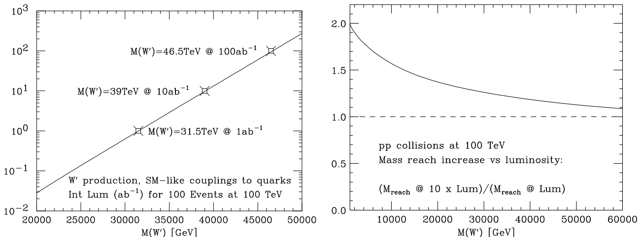
Figure 1: Left plot: integrated luminosity ( \text{ab}^{-1} ) required to produce 100 events of a sequential standard-model W' boson at 100 TeV, as a function of the W' mass. Right plot: mass reach increase for a sequential W' from a factor of 10 increase in luminosity.
