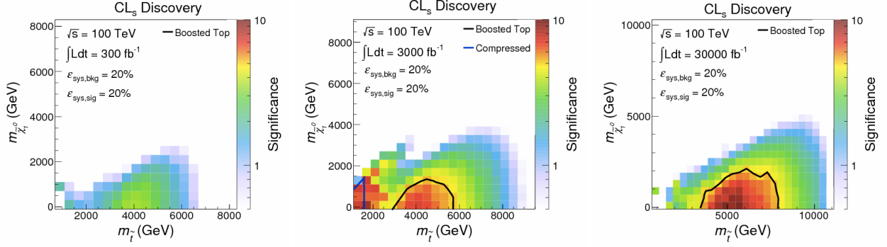
Figure 5: Top squark signal efficiency at 100 TeV, with 0.3, 3 and 30 \text{ab}^{-1} (left to right, respectively), from Ref. [13]
