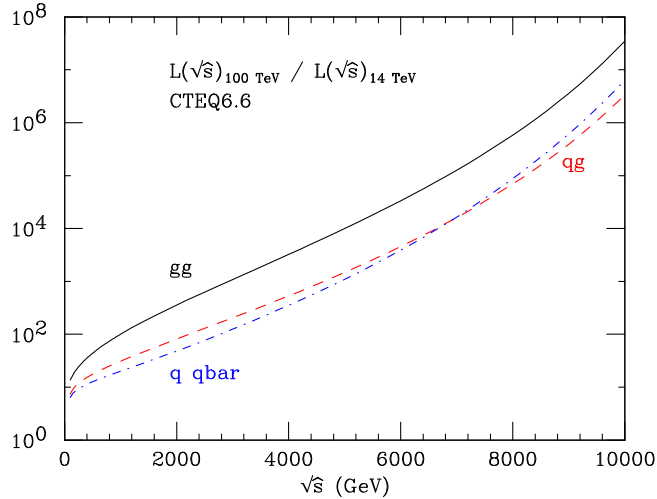
Figure 6: Ratio of partonic luminosities at 100 and 14 TeV, as a function of partonic center-of-mass energy \sqrt{\hat{s}} , for different partonic initial states. PDF set CTEQ6.6 [14], Q^2 = \hat{s} .
