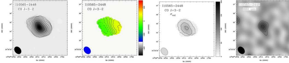
Fig. 5.— IRAS 10565 CO J=3-2 and 880 \mu\text{m} continuum maps. Notation as in Figure 2. (a) CO J=3-2 moment 0 map. Lowest contour is 2\sigma = 4.3 \text{ Jy beam}^{-1} \text{ km s}^{-1} and contours increase by factors of 1.5. (b) CO J=3-2 moment 1 map. Contours are 20 \text{ km s}^{-1} \times (-2, -1, 0, 1, 2, 3, 4) relative to cz . (c) CO J=3-2 moment 2 map. Contours are 20 \text{ km s}^{-1} \times (1, 2, 3) . (d) Uncleaned 880 \mu\text{m} map. Lowest contour is 2\sigma = 5.4 \text{ mJy} and contours increase in steps of 1\sigma . A residual sidelobe can be seen at the eastern edge of this figure.
