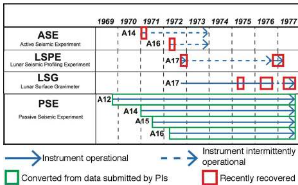
Fig. 2 Overview of the operating periods of the Apollo seismic experiments, and data availability. Solid blue lines indicate mainly operational instruments (with just occasional outages and data loss). Dashed lines indicate instruments which were mostly on standby but were occasionally turned on in their listening mode. Additional passive seismic data are available from Apollo 11 from 21 July to 3 August 1969 and again from 19 to 26 August 1969. After Nagihara et al. (2017)
