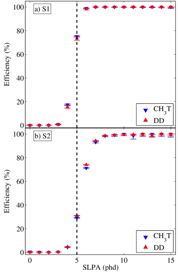
Figure 7: Measured trigger efficiencies as a function of the SLPA. The results from CH 3 T and DD data sets are compared. a) The S2 filter trigger efficiency for S1 ( \mathcal{E}_{S1}(SLPA) ). b) The S2 filter trigger efficiency for S2 ( \mathcal{E}_{S2}(SLPA) ). The vertical dashed lines represent the low filter threshold of 5 phd.
