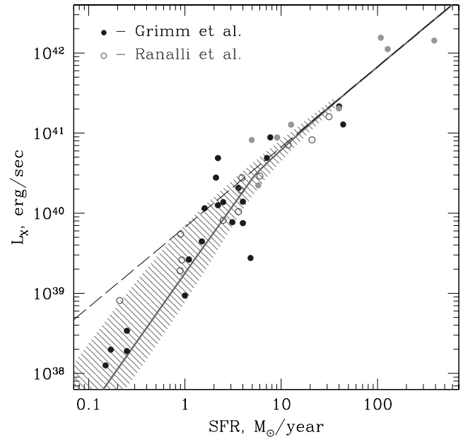
Figure 4. L_X -SFR relation. The data used is the combined data from Ranalli et al. (2003) and Grimm et al. (2003), with duplications excluded. The L_X values for nearby galaxies were corrected for the LMXB contribution estimated from the stellar mass. Three galaxies with more than 50 per cent LMXB contribution and small stellar mass, M_* < 2 \times 10^{10} M_\odot , for which large intrinsic dispersion of the L_X - M_* relation precludes accurate estimate of the LMXB luminosity are not plotted. The luminosities for the HDF-N and Lynx field galaxies were computed for H_0 = 70 \text{ km s}^{-1} \text{ Mpc}^{-1} , \Omega_m = 0.3 , \Lambda = 0.7 . The solid and dashed lines and the shaded area are the same as in Fig. 1. This figure is available in colour in the online version of the journal on Synergy .
