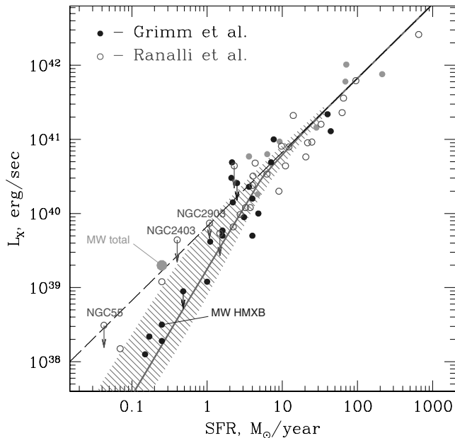
Figure 1. L_X –SFR relation. All points are from Ranalli et al. (2003) and Grimm et al. (2003) are plotted. The galaxies with the expected LMXB fraction exceeding 50 per cent are plotted as upper limits. The thick solid line shows the predicted relation between the most probable values of L_X and the SFR; the shaded area indicates its 67 per cent intrinsic spread. The straight dashed line shows the expectation mean for L_X , which would be obtained if X-ray luminosities of many galaxies with similar SFR were averaged. To demonstrate the importance of the LMXB contribution at low SFR/ M_* , both HMXB and total luminosities are plotted for the Milky Way. This figure is available in colour in the online version of the journal on Synergy .
