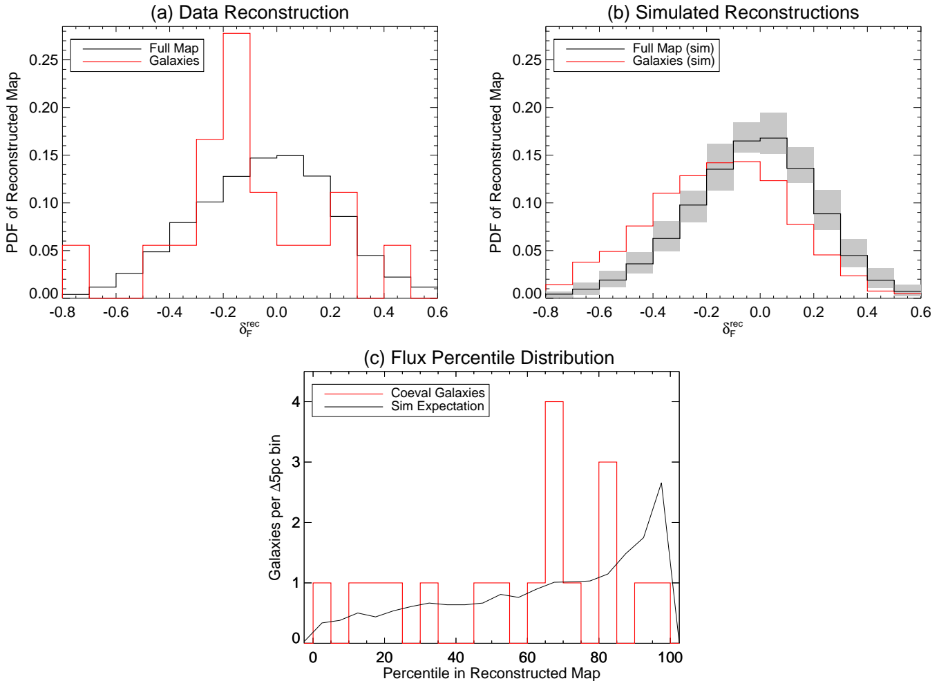
FIG. 5.— (a) PDF of our tomographic map (black) compared with that sampled by 18 coeval galaxies within our map volume (red, both PDFs normalized to unit area). (b) Similar to (a), but evaluated over 24 mock reconstructions simulating the real map. The red curve shows the \delta_F^{\text{rec}} evaluated at 2506 simulated R \leq 25.5 galaxies within the mock reconstructions — the simulated galaxies clearly also preferentially live in low- \delta_F^{\text{rec}} regions. Shaded regions indicate the range of map PDFs from the 24 mock reconstructions, indicating the significant sample variance from the small volume. (c) Distribution of coeval galaxies as a function of the map flux percentile, such that \delta_F^{\text{rec}} decreases with the percentile, i.e. larger percentiles probe overdensities. The black curve indicates the predicted distribution from the simulated galaxies within our mock reconstructions.
