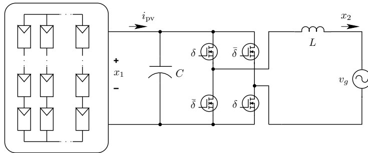
Fig. 1: Full-bridge grid-connected PV inverter schematic.
