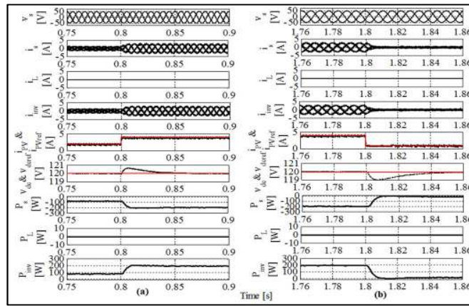
Fig. 9. Dynamic response of the DC/AC inverter under: a) increasing load and solar irradiation, and b) decreasing load and solar irradiation.
