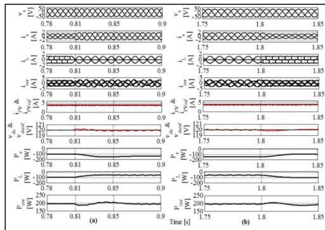
Fig. 10. Dynamic response of the DC/AC inverter under nonlinear loads (a) fixed solar irradiation and switching off load on phase 'a' at t=0.81s (b) fixed solar irradiation and switching on load on phase 'a' at t=1.8s.
