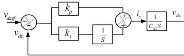
Fig. 6. Transfer function of the DC link voltage regulation.
