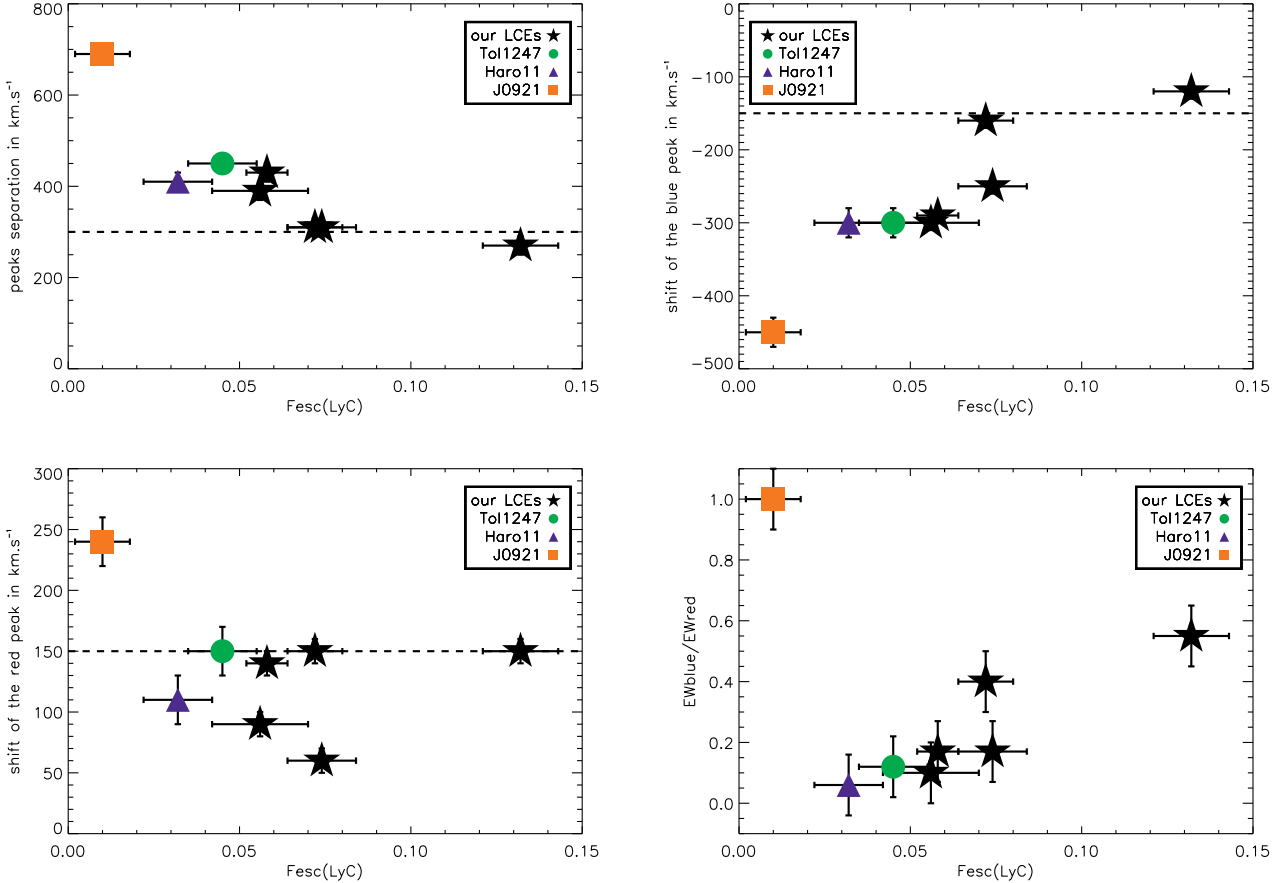
Fig. 5. Comparison of the Ly \alpha diagnostics for LyC leakage with the escape fraction of ionizing photons. The correlation between the peak separation and the escape fraction of ionizing photons is driven by the shift of the blue peak back to line center. The dashed lines correspond to the theoretical predictions for f_{\text{esc}}^{\text{LyC}} \sim 30\% ( \tau_{\text{LyC}} \sim 1 ) from Verhamme et al. (2015).
