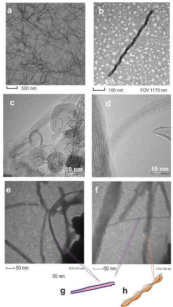
Fig. 3. a) LVTEM image of LAF and b) fibril detail, c) TEM image of SWCNT and d) SWCNT detail e, f) LVTEM images of LAF+SWCNT g) schematic illustration of the SWCNT structure h) schematic illustration of the fibril structure.
