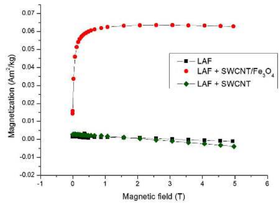
Fig. 2. Magnetization curves of a) LAF, b) LAF+SWCNT, c) LAF+SWCNT/ \text{Fe}_3\text{O}_4 .
