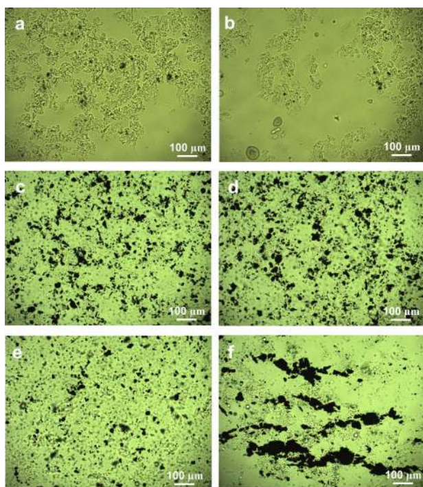
Fig. 4. POM images of a) LAF, b) LAF in external magnetic field of 1.5T c) LAF+SWCNT, d) LAF+SWCNT in external magnetic field of 1.5T, e) LAF+SWCNT/Fe 3 O 4 f) LAF+SWCNT/Fe 3 O 4 in external magnetic field of 1.5 T.
