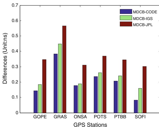
Fig. 5 The mean differences between receiver DCB values estimated by M_DCB and those released by CODE, JPL, and IGS combined
