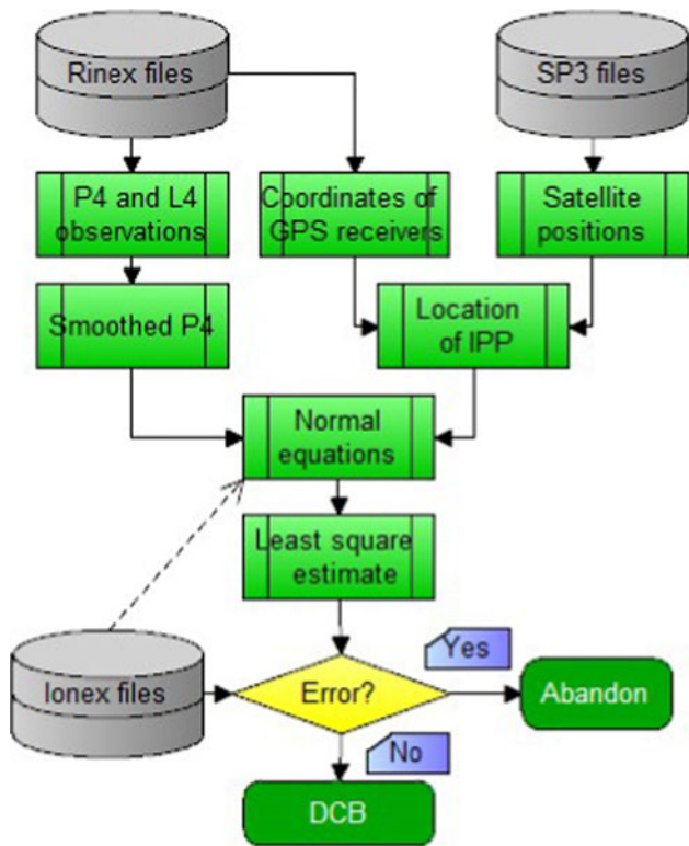
Fig. 1 Flowchart of M_DCB software
