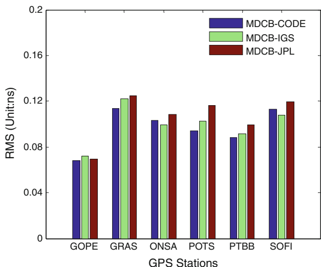
Fig. 6 The RMSs of the differences between receiver DCB values estimated by M_DCB and those released by CODE, JPL, and IGS combined
