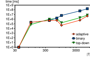
Fig. 11. Runtime of adaptive and non-adaptive m -privacy verifications vs. |T| (log-log scale).
