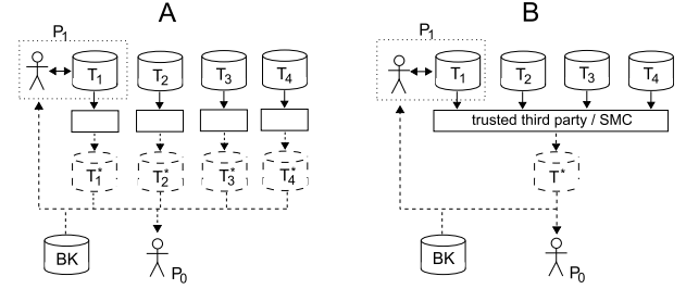
Fig. 1. Distributed data publishing settings.
