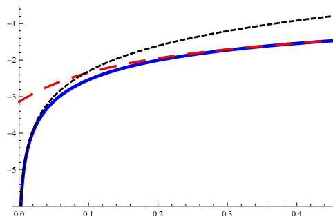
Figure 2. Comparison of the exact result for d^2F_0/d\lambda^2 given in (3.34), and plotted in a continuous blue line, with the strong and weak coupling behavior. The red dashed line represents the strong coupling behavior (3.55), while the black dashed line represents the Gaussian weak coupling behavior (3.33).
